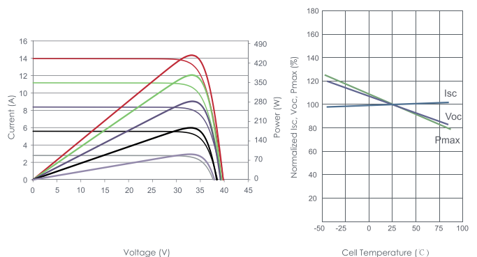
Temperatura celdas | Cells temperature: 25°C. Current-Voltage & Power Voltage Curve (435)
