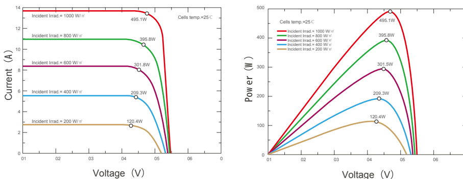
Temperatura celdas | Cells temperature: 25°C. Current-Voltage & power Voltage Curve (505)
