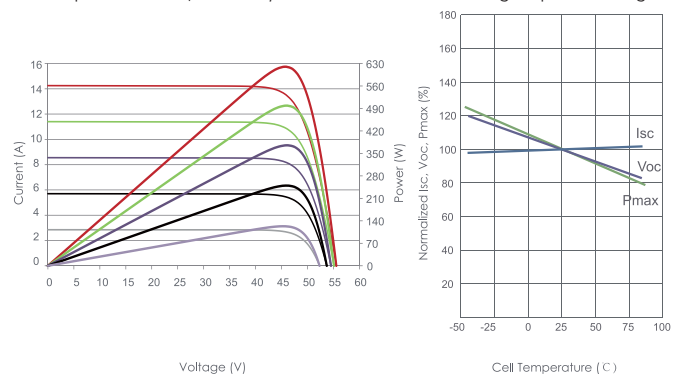
Temperatura cella | Cells temperature: 25°C. Current-Voltage & power Voltage Curve
